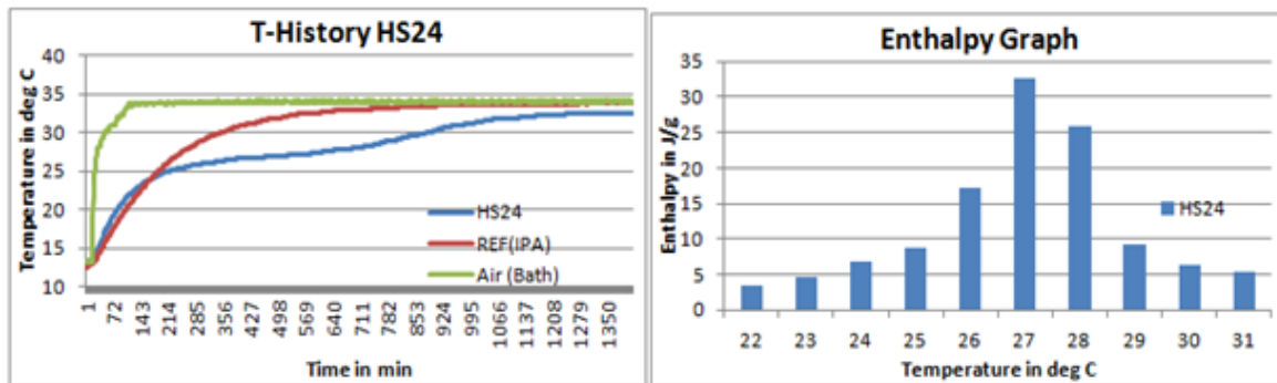
Fig1: T-History graph for HS24 done in air bath
