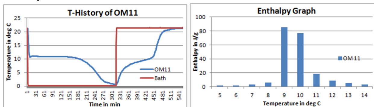
Fig1: T-History graph for OM11 done in air bath
