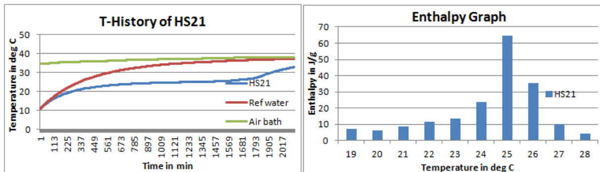
Fig1: T-History graph for HS21 done in air bath
