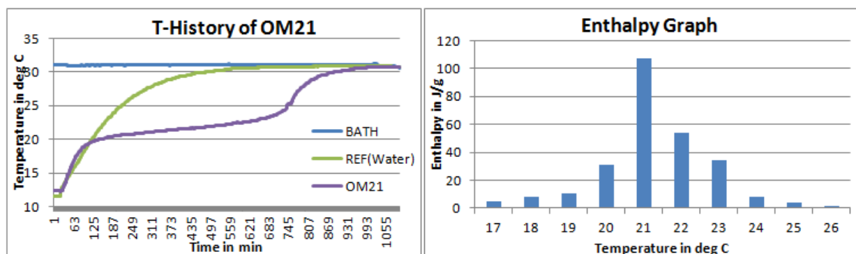
Fig1: T-History graph for OM21 done in air bath
