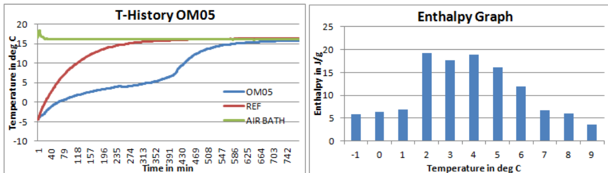
Fig1: T-History graph for OM05 done in air bath
