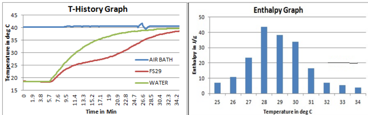
Fig1: T-History graph for FS29 done in air bath
