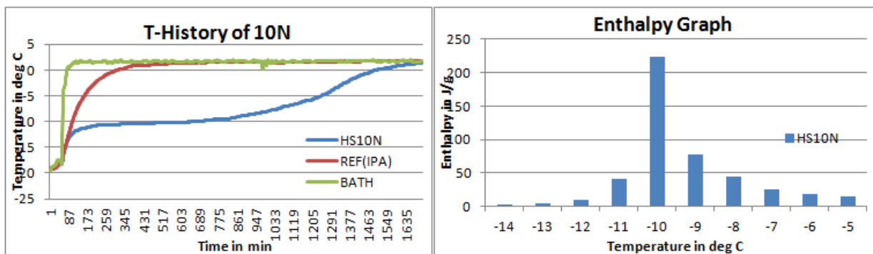
Fig1: T-History graph for HS10N done in air bath
