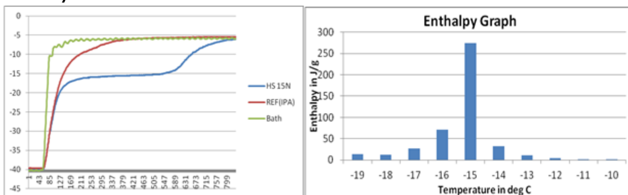
Fig1: T-History graph for HS15N done in air bath
