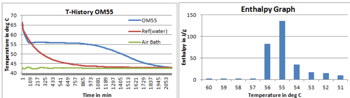
Fig1: T-History graph for OM55 done in air bath
