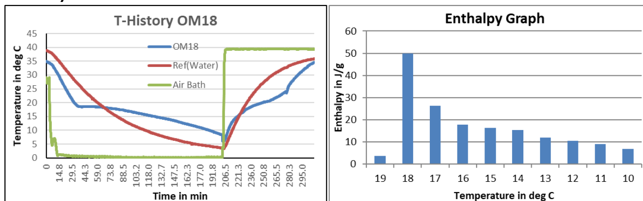
Fig1: T-History graph for OM18 done in air bath
