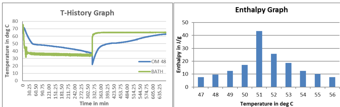
Fig 1: T-history Method of OM48
