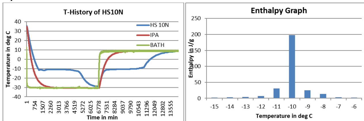
Fig1: T-History graph for HS10N done in air bath
