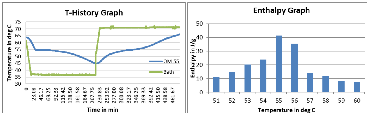
Fig1: T-History graph for OM55
