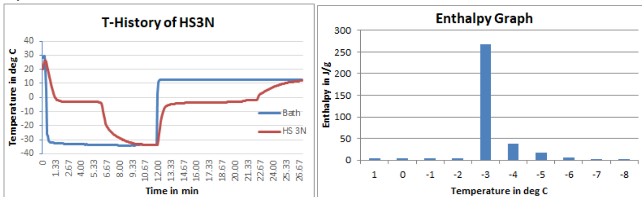
Fig1: T-History graph for HS3N
