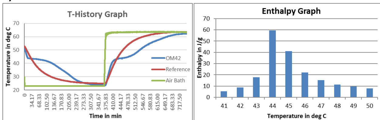
Fig1: T-History graph for OM42
