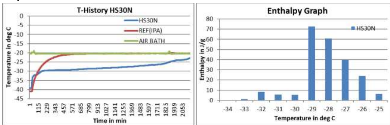
Fig1: T-History graph for HS30N done in air bath
