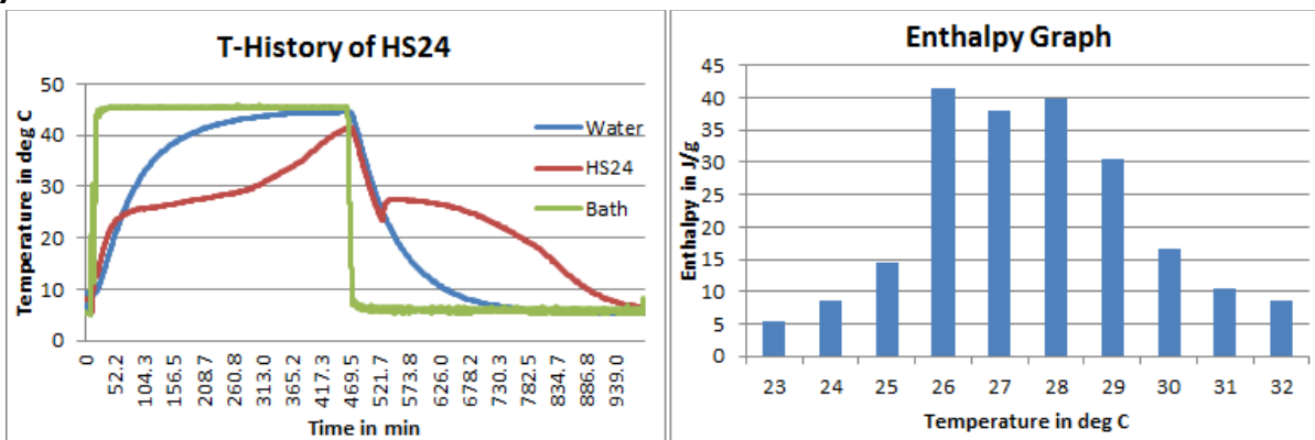
Fig1: T-History graph for HS24 done in air bath
