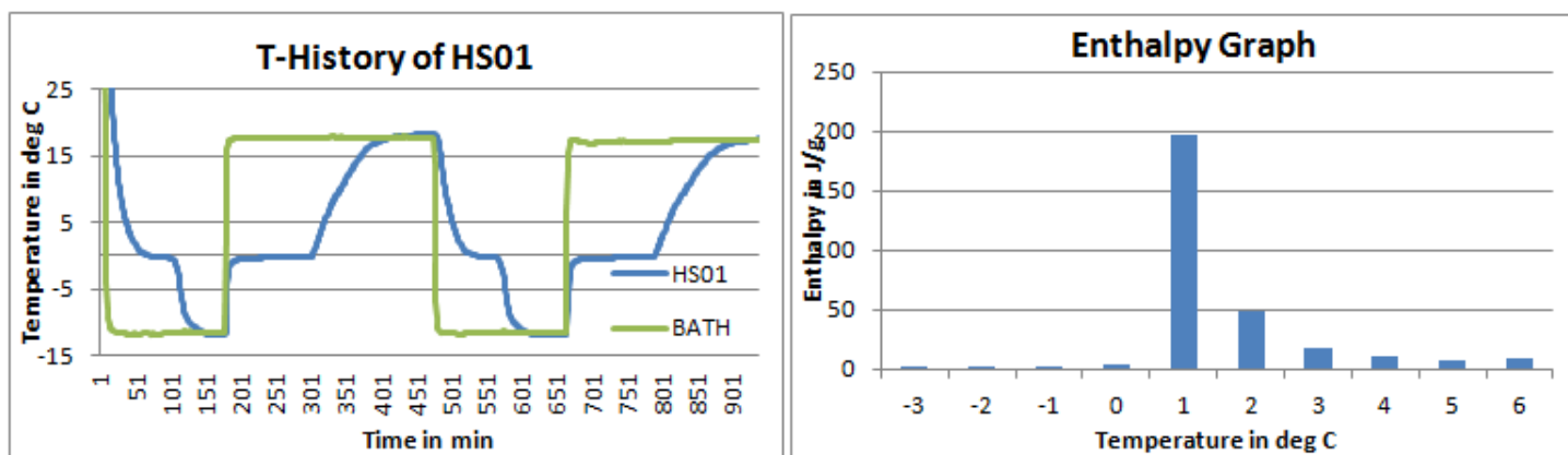
Fig 1: T-History graph of HS01/I in air bath
