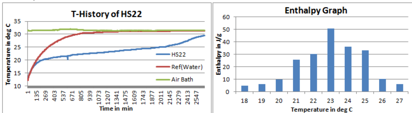
Fig 1: T-History graph of HS22 in Air Bath
