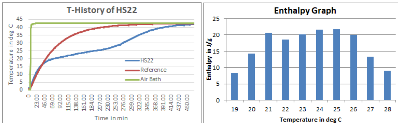
Fig 1: T-History graph of HS22 in Air Bath
