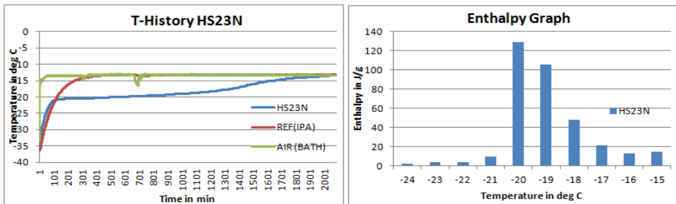
Fig1: T-History graph for HS23N done in air bath
