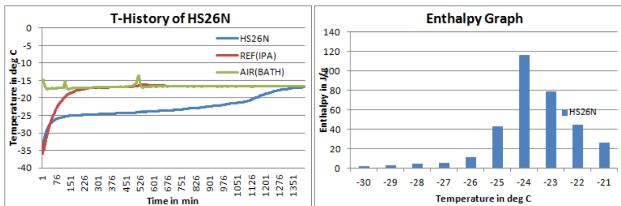
Fig1: T-History graph for HS26N done in air bath
