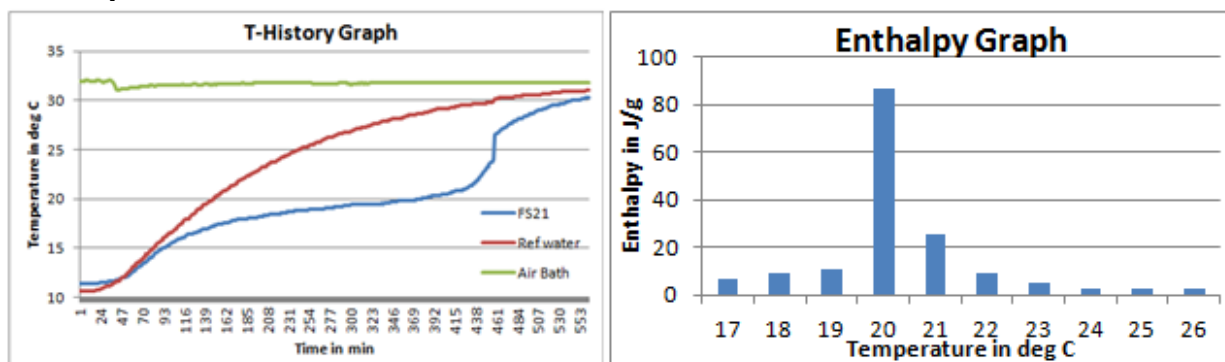
Fig1: T-History graph for FS21 done in air bath
