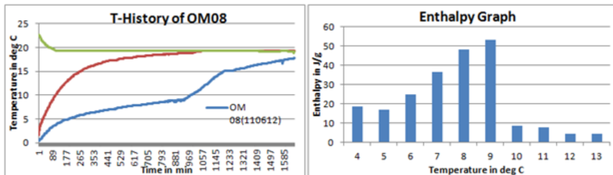
Fig1: T-History graph for OM08 done in air bath
