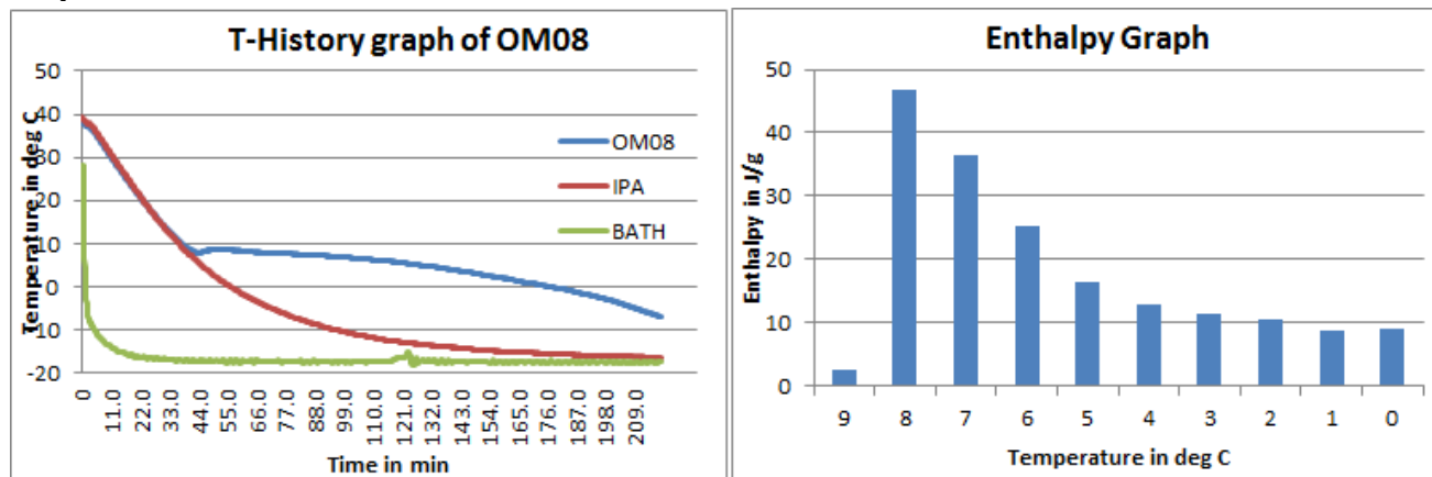
Fig1: T-History graph for OM08 done in air bath
