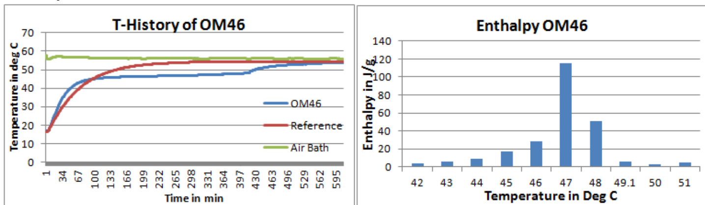
Fig 1: T-History Graph of OM46 in Air Bath
