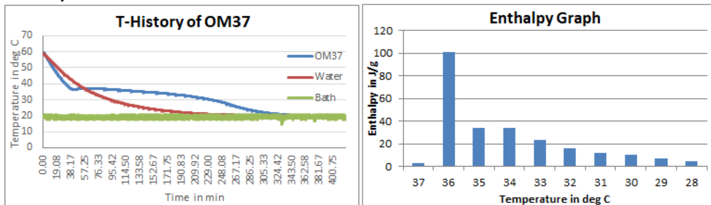
Fig 1: T-History graph of OM37 in Air Bath
