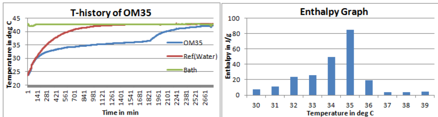
Fig 1: T-History graph of OM35 in Air Bath
