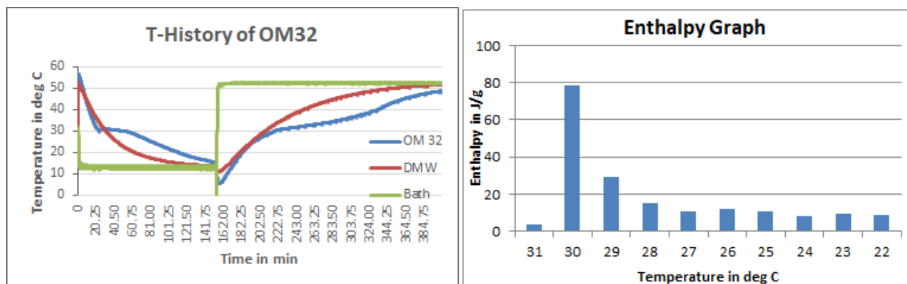
Fig 1: T-history graph of OM32 in Water bath
