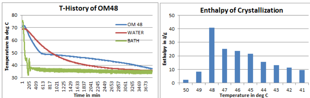
Fig 1: T-history Method of OM48
