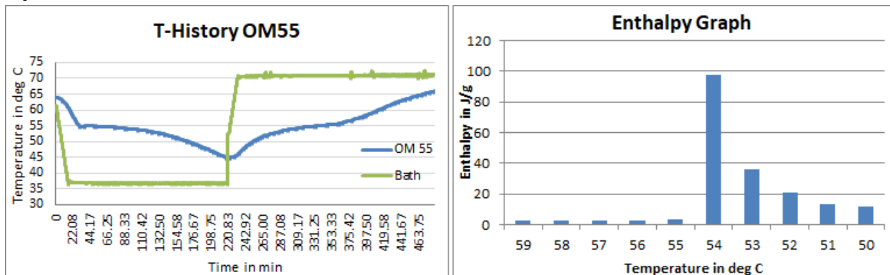
Fig1: T-History graph for OM55 done in air bath
