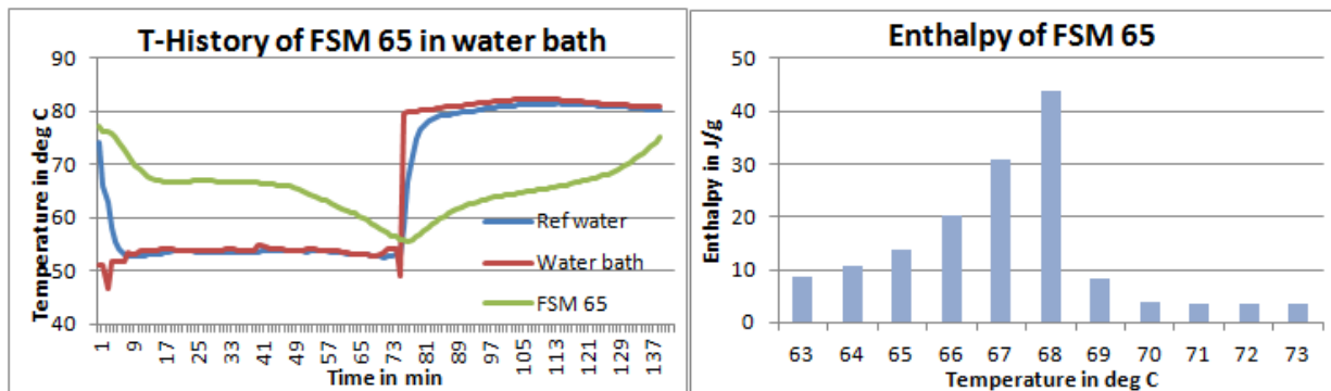
Fig1: T-History graph for FSM65 done in air bath
