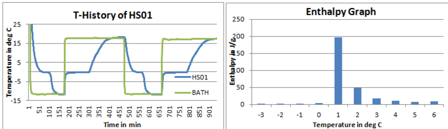
Fig 1: T-History graph of HS01 in air bath
