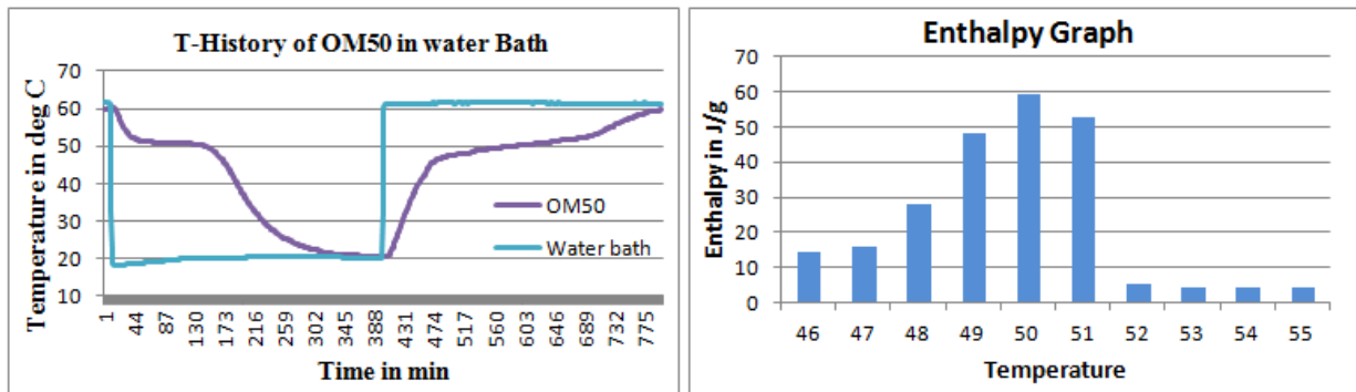
Fig1: T-History graph for OM50 done in water bath
