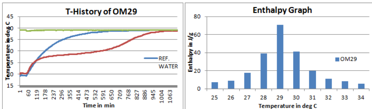
Fig1: T-History graph for OM29 done in air bath
