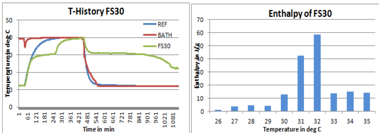
Fig1: T-History graph for FS30 done in air bath
