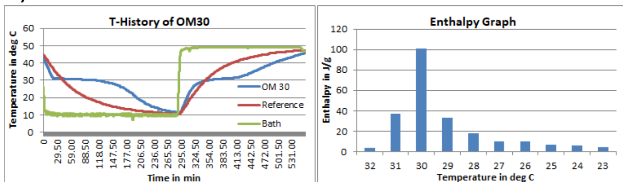
Fig1: T-History graph for OM30 done in water bath
