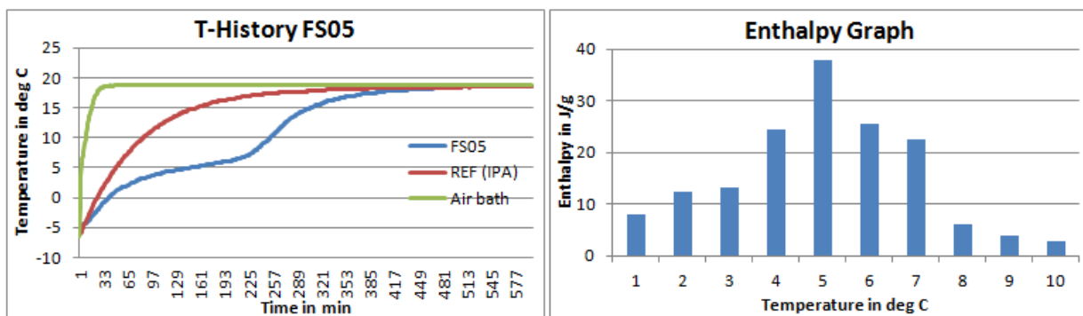
Fig1: T-History graph for FS05 done in air bath
