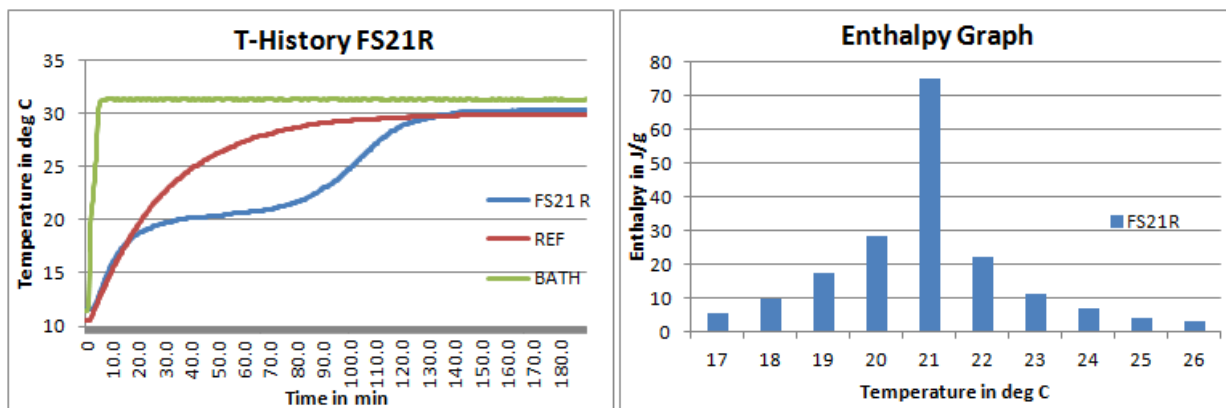
Fig1: T-History graph for FS21R done in air bath
