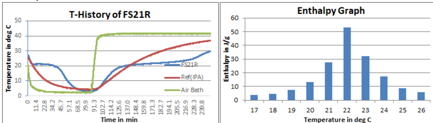
Fig1: T-History graph for FS21R done in air bath
