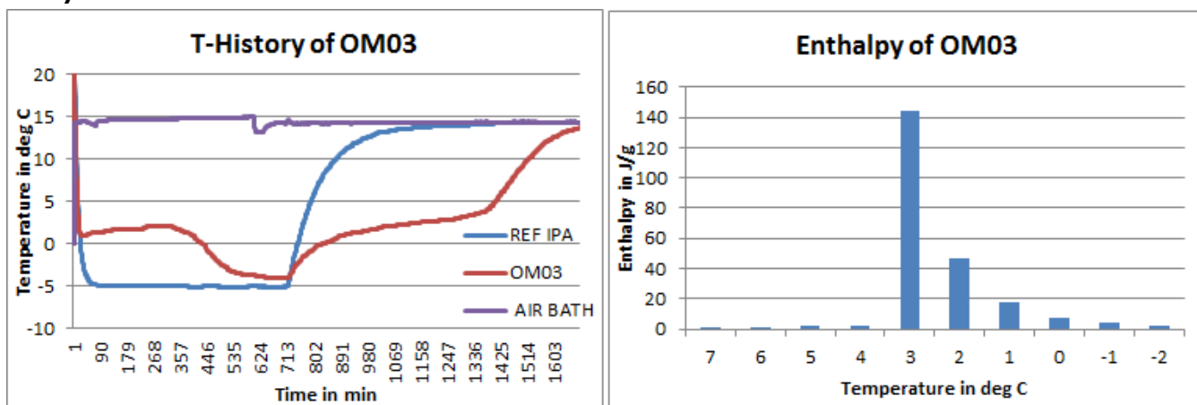
Fig1: T-History graph for OM03 done in air bath
