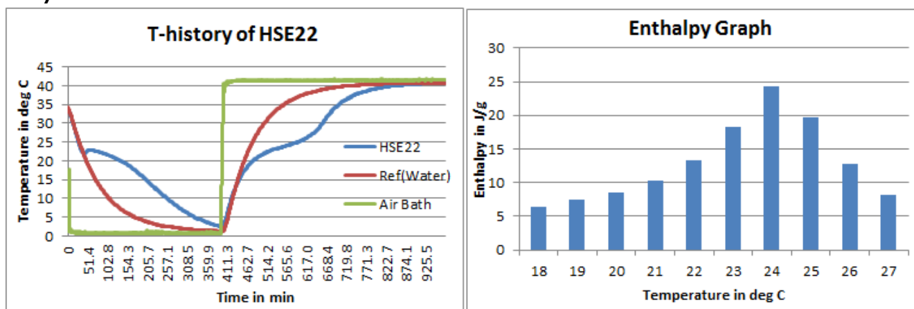
Fig1: T-History graph for HSE22 done in air bath
