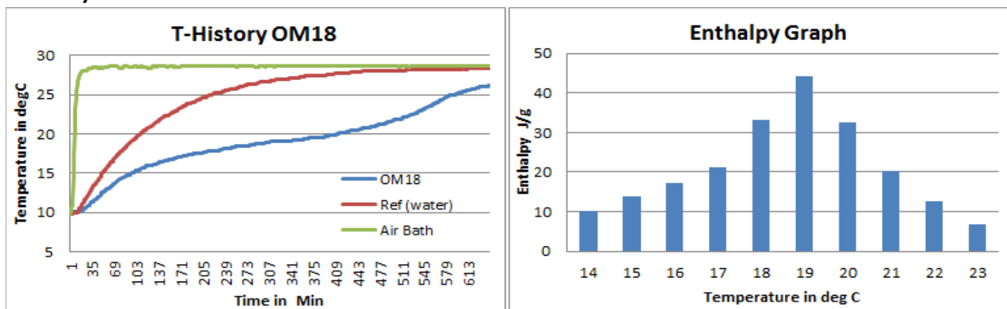
Fig1: T-History graph for OM18 done in air bath
