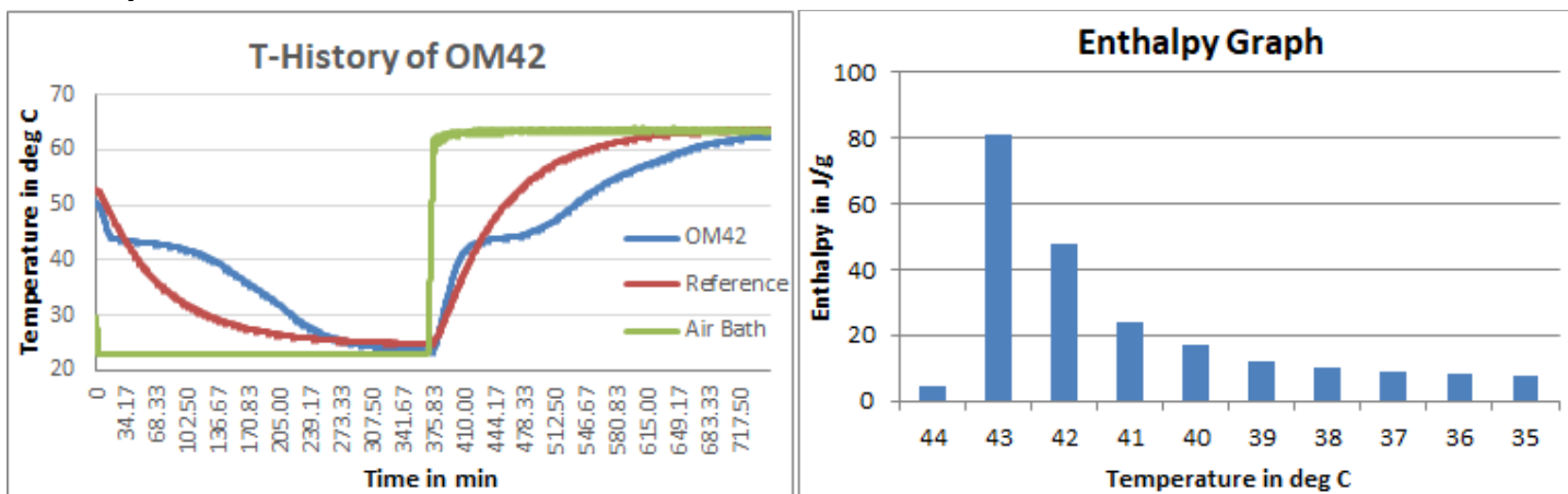
Fig1: T-History graph for OM42 done in air bath
