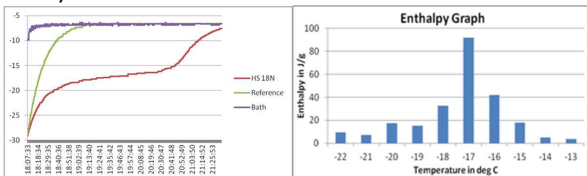
Fig1: T-History graph for HS18N done in air bath
