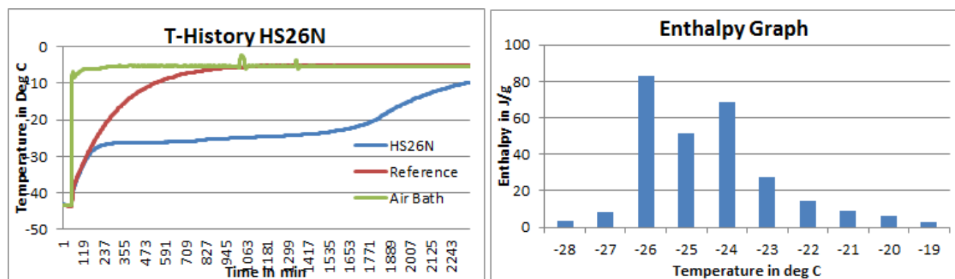
Fig1: T-History graph for HS26N done in air bath
