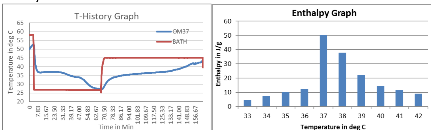
Fig 1: T-History graph of OM37 in Air Bath
