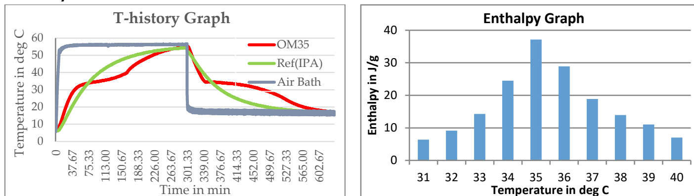
Fig 1: T-History graph of OM35 in Air Bath
