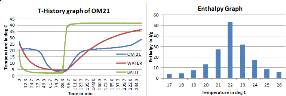
Fig1: T-History graph for OM21 done in air bath
