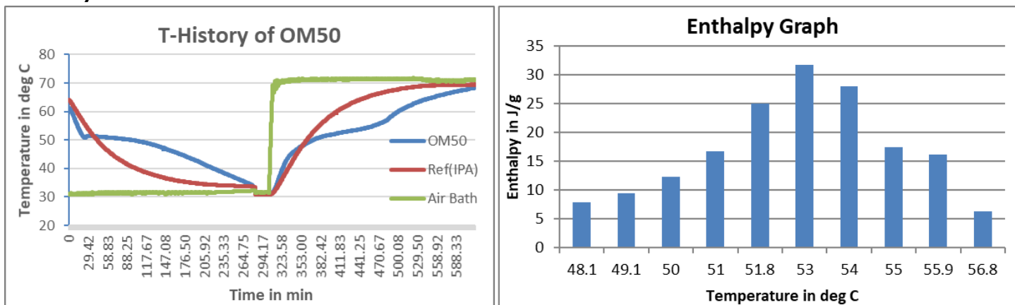
Fig1: T-History graph for OM50
