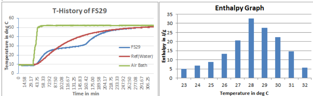
Fig1: T-History graph for FS29 done in air bath
