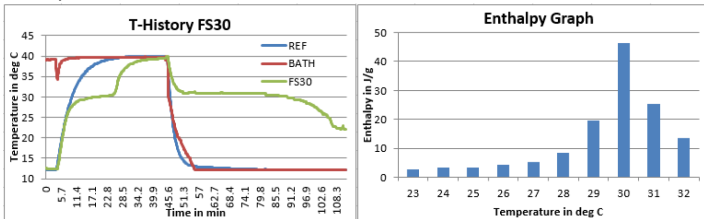
Fig1: T-History graph for FS30 done in air bath
