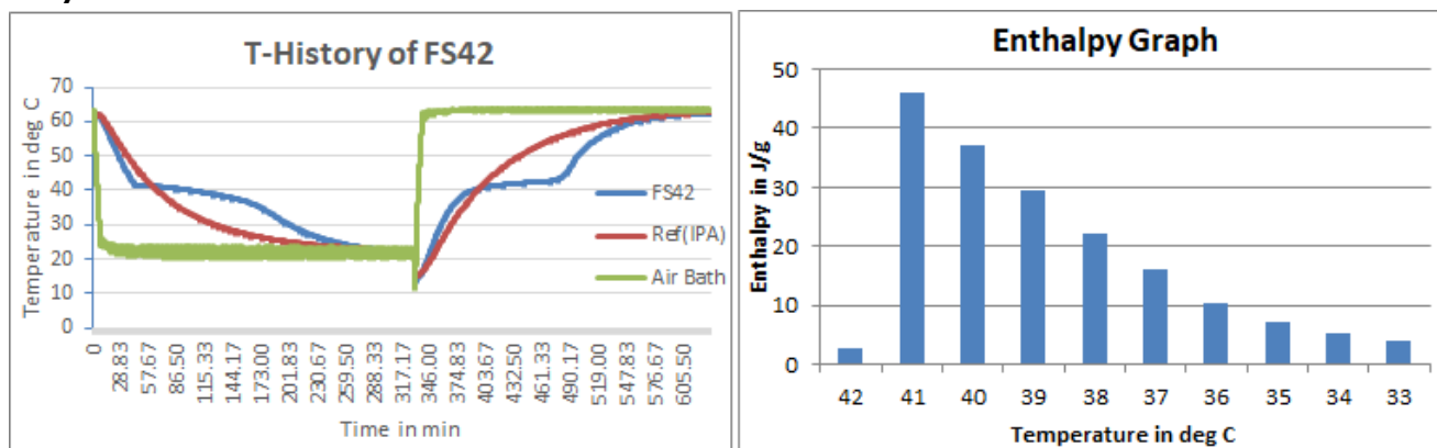
Fig1: T-History graph for FS42 done in air bath
